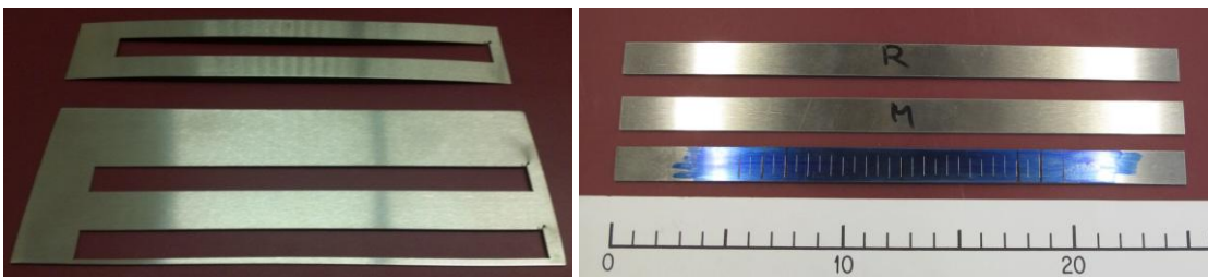
Figure 2. Left: original 50 \times 0.5 \text{ mm}^2 and 100 \times 1.5 \text{ mm}^2 strips with cut out samples. Right: Fe-SMA strips before the tensile test, marks for the strain measurements. (dimensions in mm).
